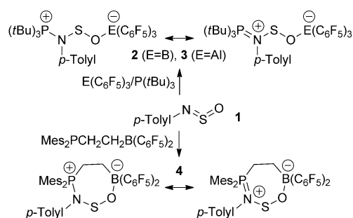
Scheme 2. Synthesis of 2–4 .
